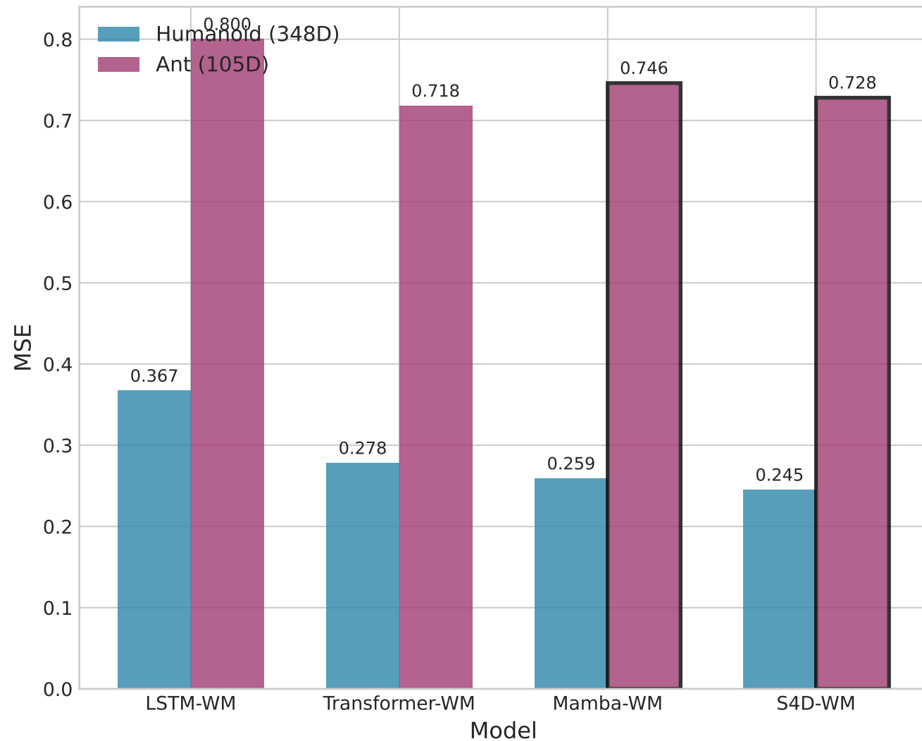
Prediction MSE on D4RL Datasets
