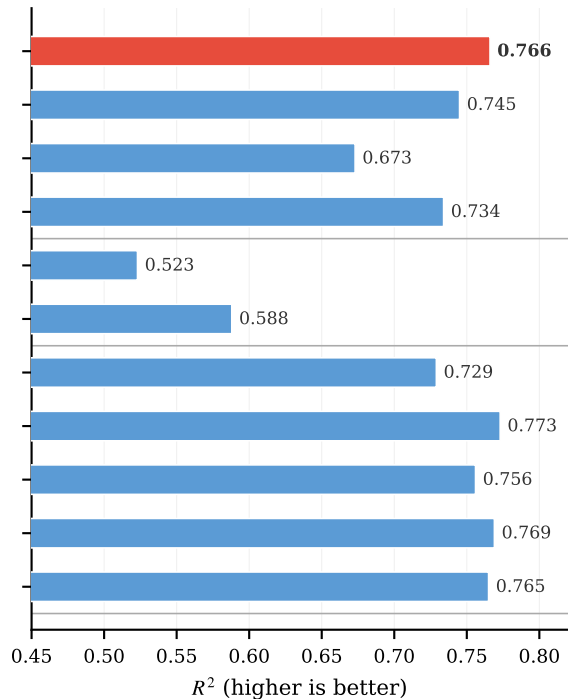
(b) R^2
