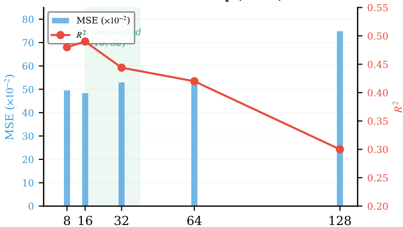
HumanoidStandup (376-D)
