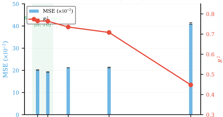
HumanoidStandup (376-D)
