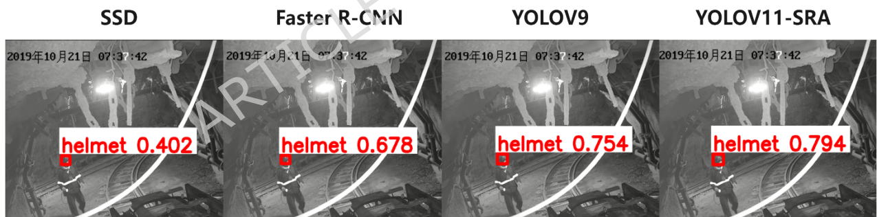
Figure 8. Comparison of model detection results in extremely low-light scenarios
