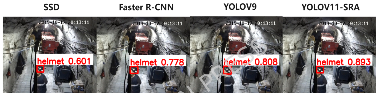
Figure 7. Comparison of Model Detection Results in Severely Occluded Scenarios
