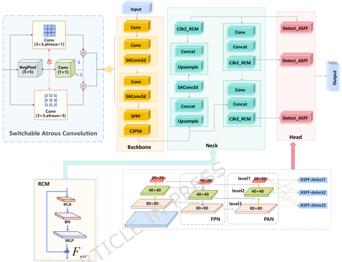
Figure 1. YOLOv11-SRA Model Architecture Diagram
