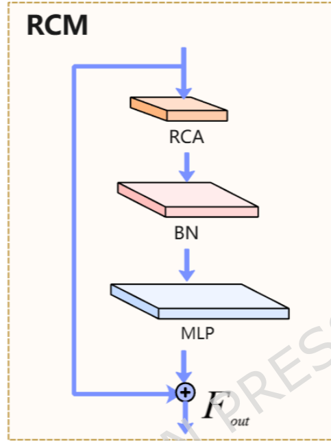
Figure 3. RCM Module Structure
