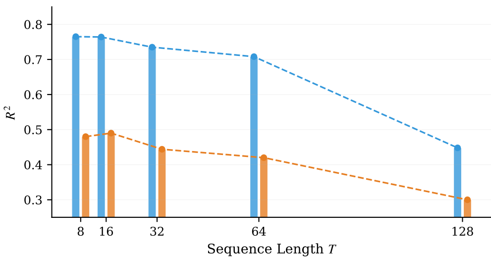
(b) R^2
