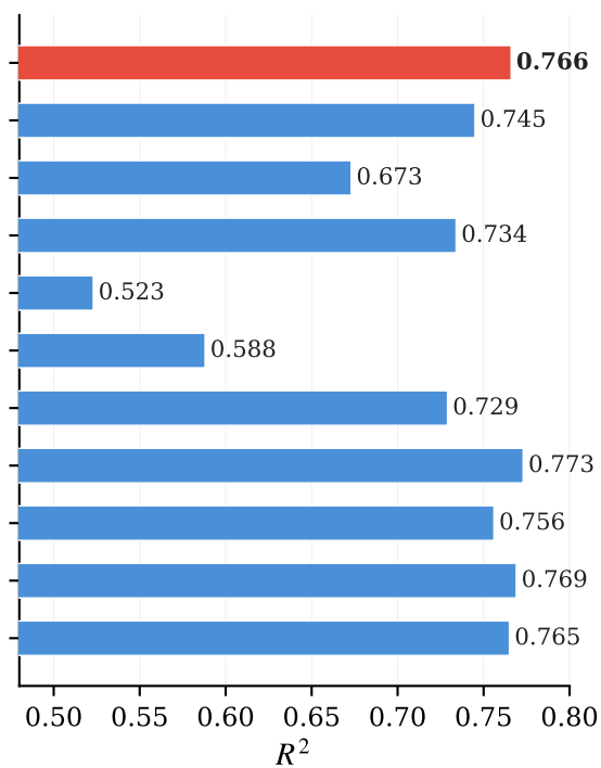
(b) R^2
