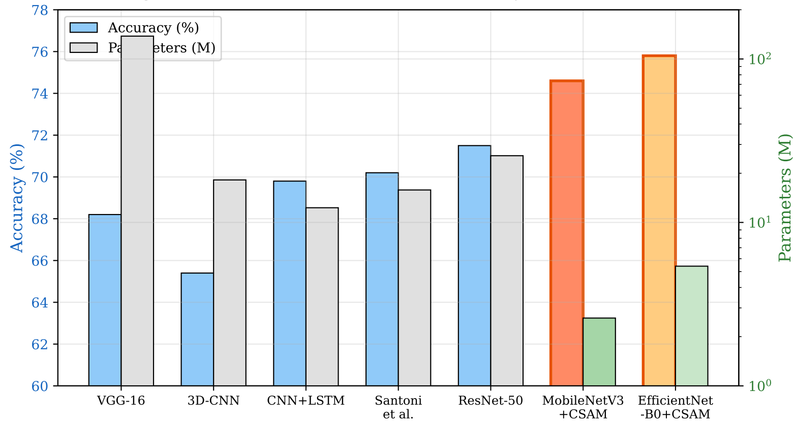
Figure 2: Model Comparison — Accuracy vs. Parameters
