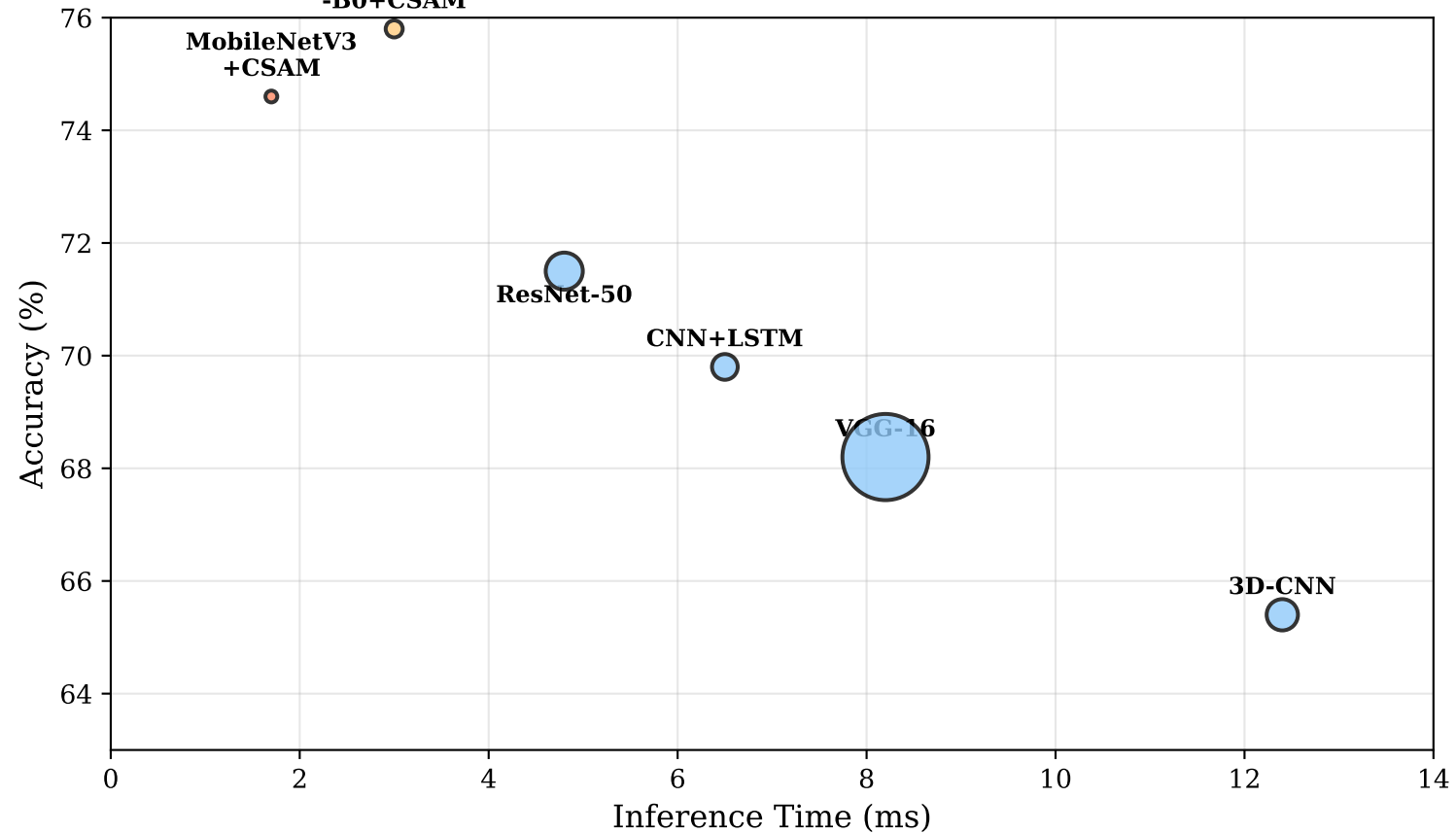
Figure 3: Efficiency vs. Accuracy (bubble size = parameters)
