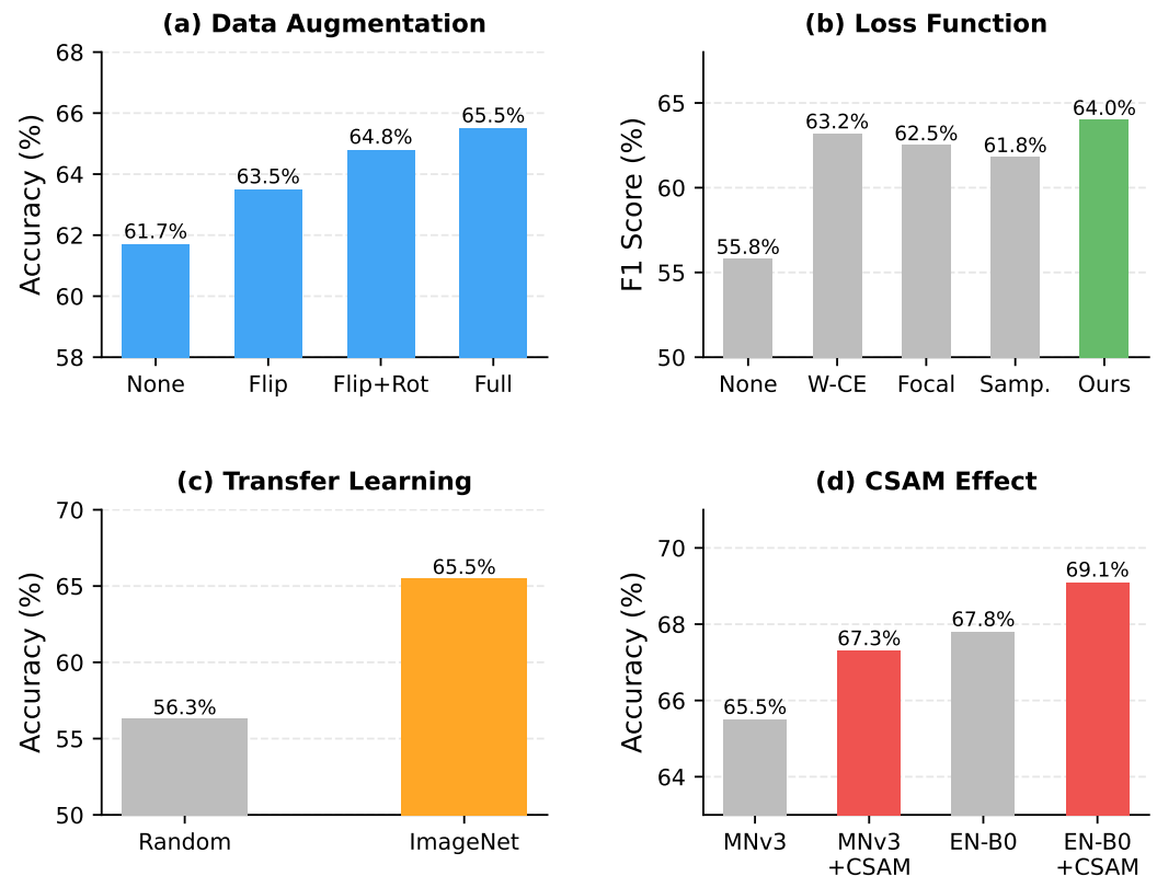
Figure 1. Ablation study results. (a) Data augmentation presets. (b) Loss function strategies (F1 score). (c) Transfer learning initialization. (d) CSAM effect on different backbones. The focal loss parameter \gamma = 1.0 was validated via a separate sensitivity analysis (Table 3).
