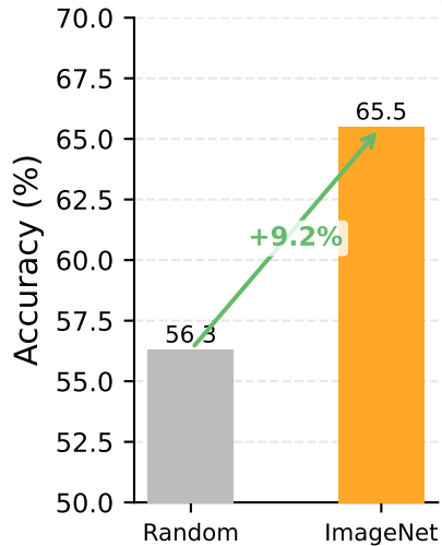
(c) Transfer Learning
