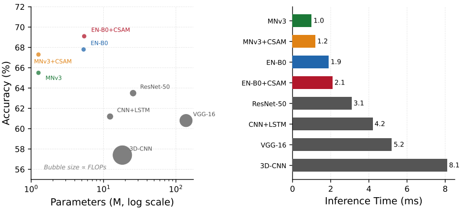
Figure 3. Efficiency-accuracy trade-off. Left: parameters vs. accuracy (bubble size proportional to FLOPs). Right: inference time comparison on RTX 3090.
