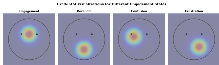
Figure 7. Grad-CAM visualizations for different engagement states. Warmer colors indicate higher attention. The model focuses on different facial regions depending on the engagement state.
