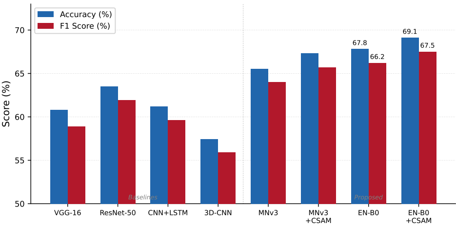
Figure 2. Comparison of accuracy and F1 score across baseline and proposed models on FER2013 engagement detection. MNv3: MobileNetV3-Small; EN-B0: EfficientNet-B0.
