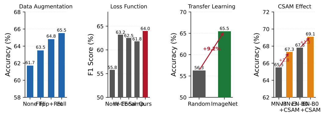
Figure 4. Ablation study results. (a) Data augmentation presets. (b) Loss function strategies (F1 score). (c) Transfer learning initialization. (d) CSAM effect on different backbones. The focal loss parameter \gamma = 1.0 was validated via a separate sensitivity analysis (Table 6).
