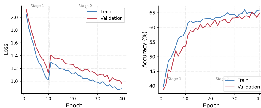
Figure 1. Training curves for MobileNetV3+CSAM on FER2013. Stage 1 (epochs 1–10): head-only training with LR=10^{-3} . Stage 2 (epochs 11–40): full fine-tuning with LR=10^{-4} .
