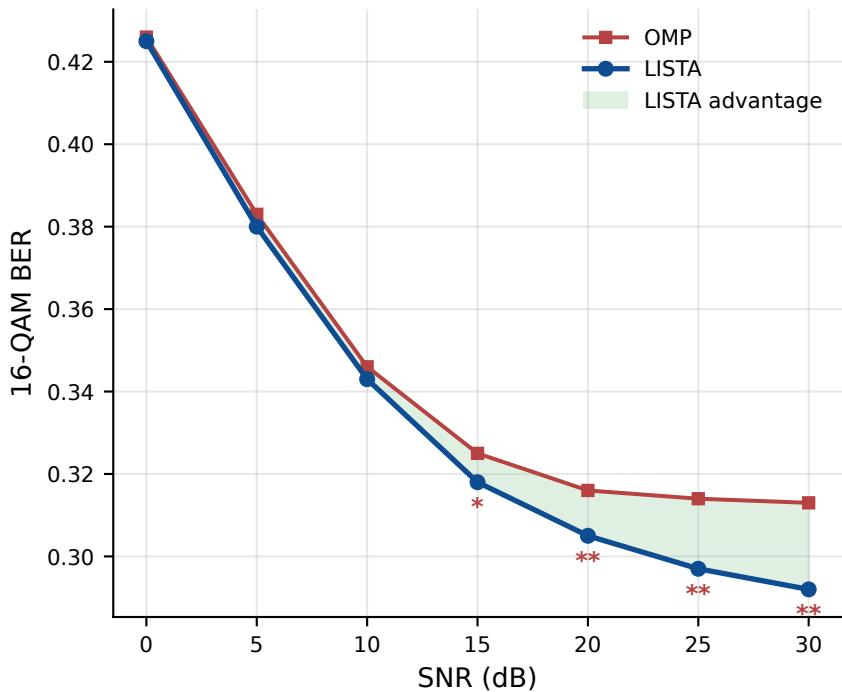
(b) BER under ZF equalization
