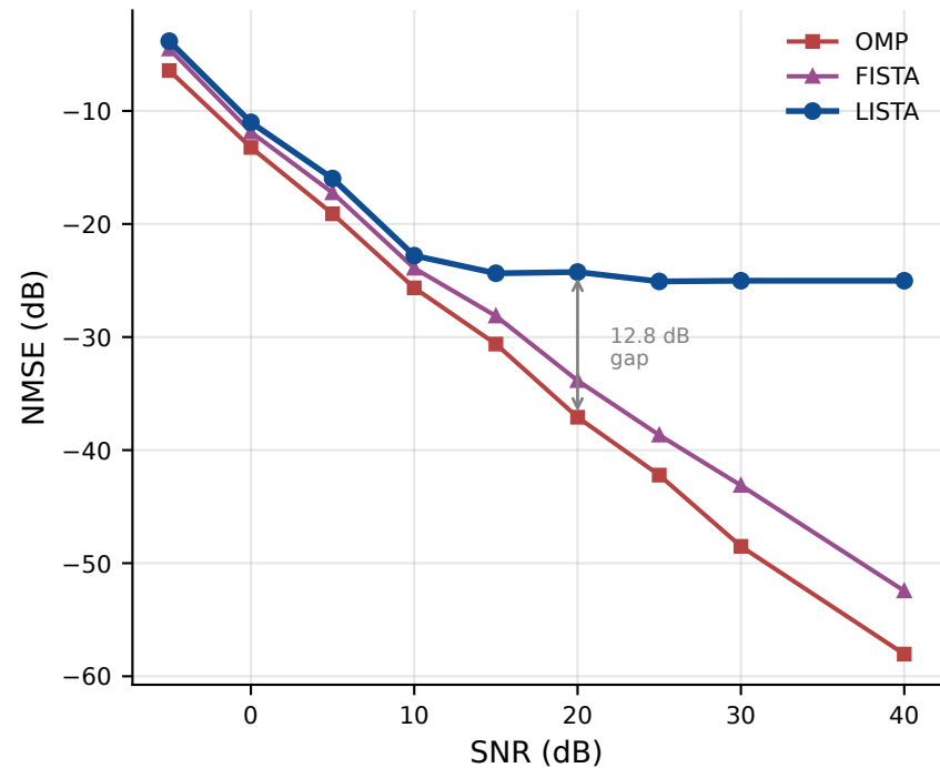
(a) NMSE vs SNR
