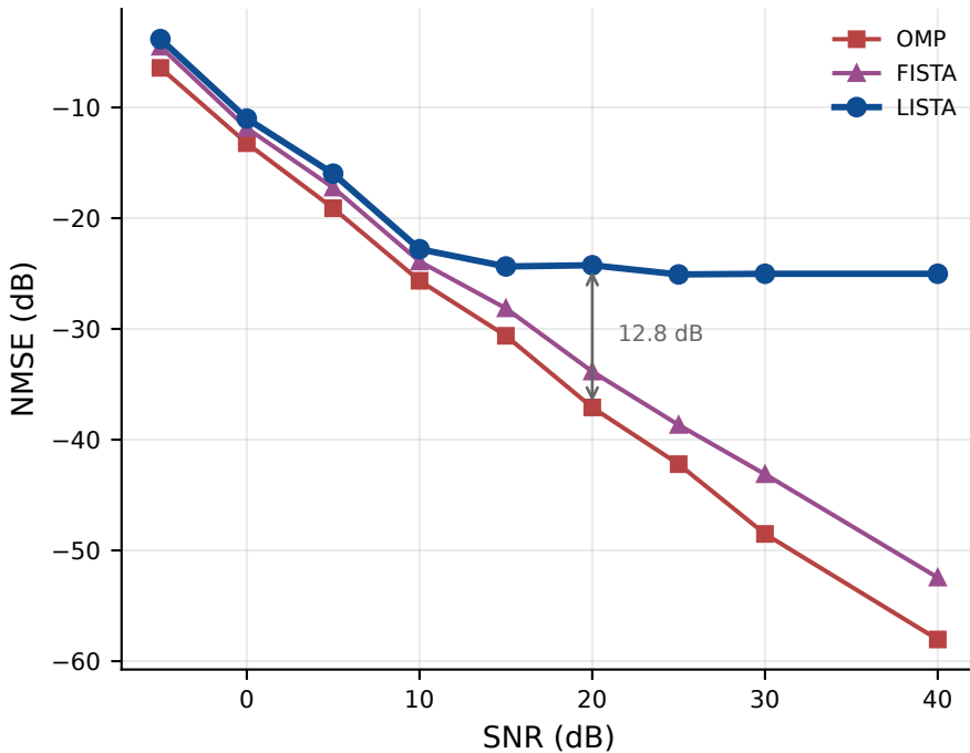
(a) NMSE vs SNR
