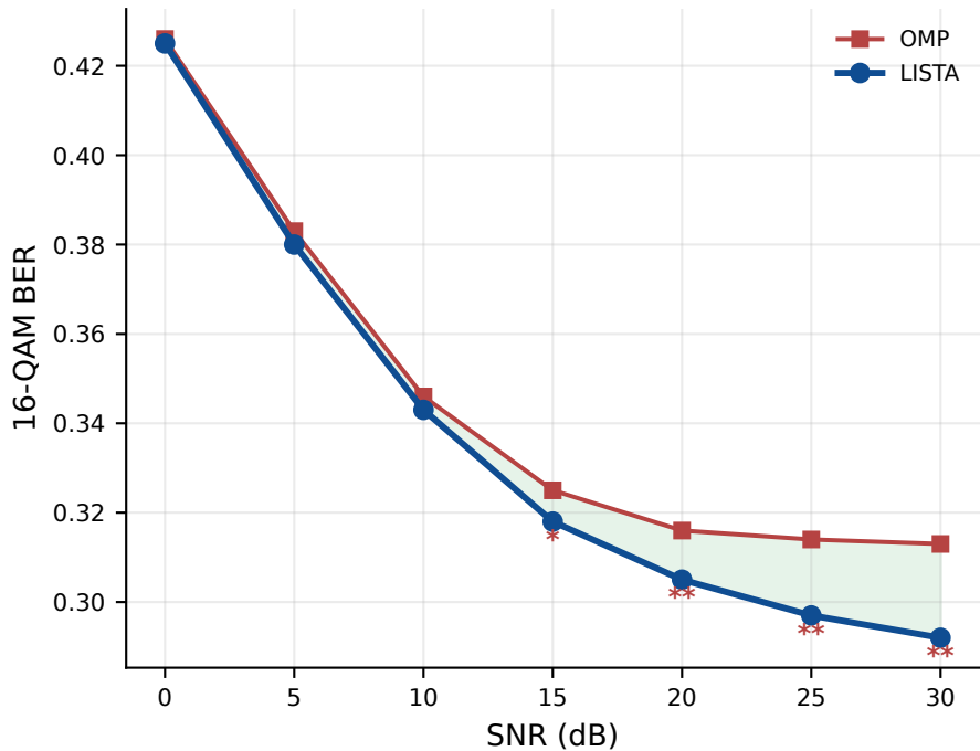
(b) BER under ZF equalization
