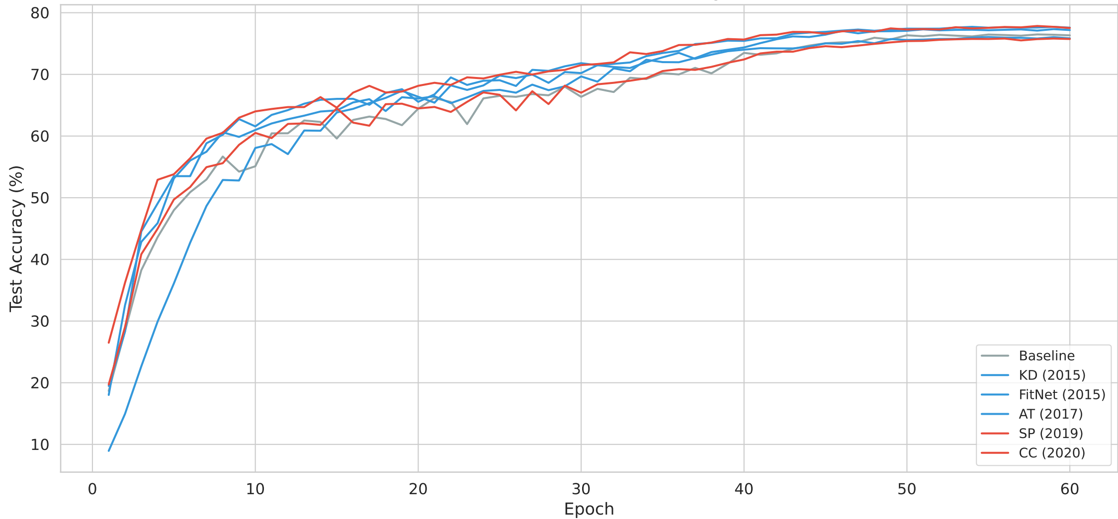
CIFAR-100: Student ResNet-18 Learning Curves
