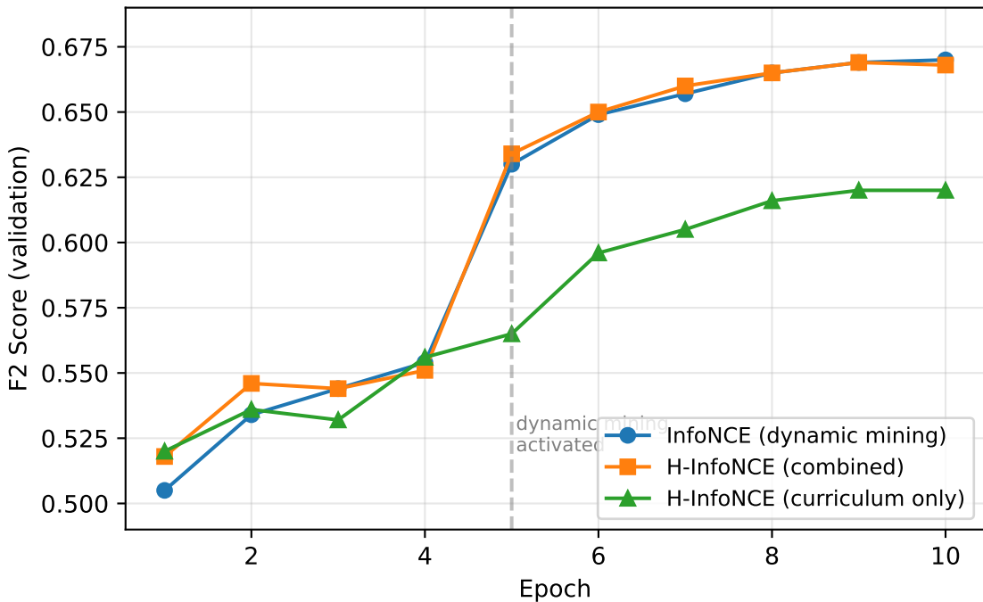
Learning Curves: Hierarchical vs. Dynamic Negative Mining
