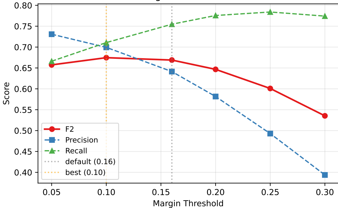
Effect of Margin Threshold on Retrieval
