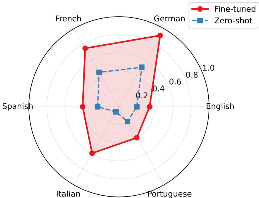
F2 Score by Language
