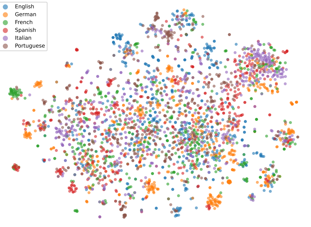
Zero-shot
