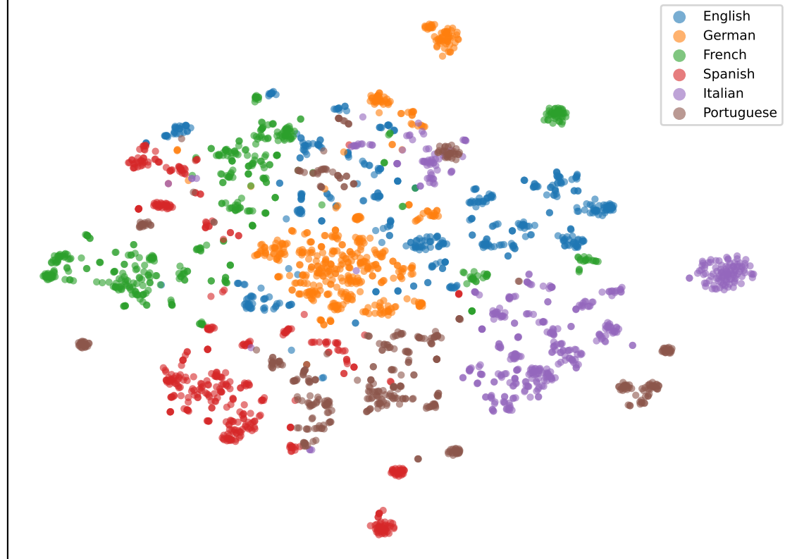
Fine-tuned
