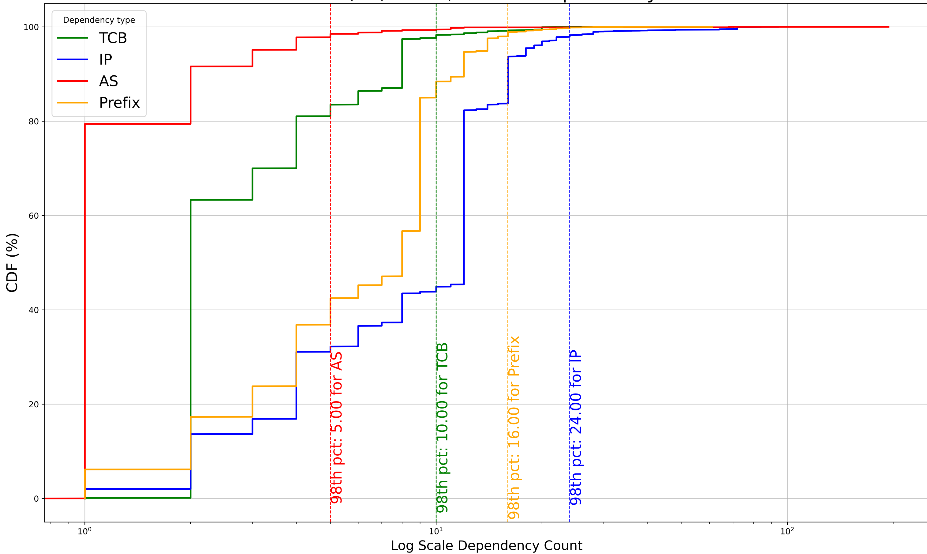
CDF of TCB, IP, Prefix, and AS Dependency Counts
