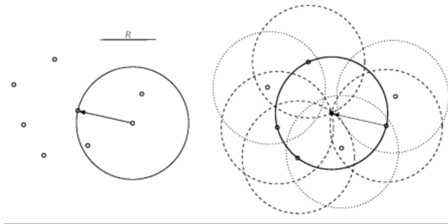
Fig. 2. Searching a circle of known radius in a point set.
