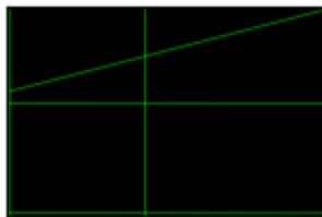
Lines
