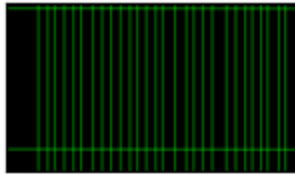
Lines
