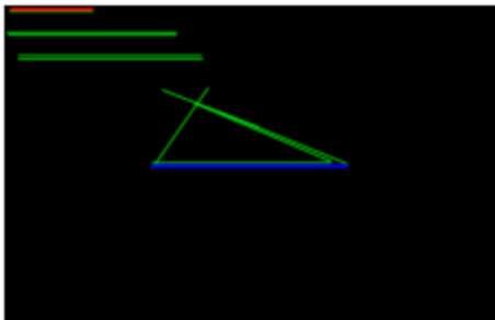
Segments
