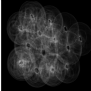
Radius 40
