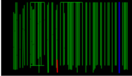
Segments
