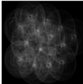
Radius 60
