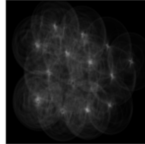
Radius 50
