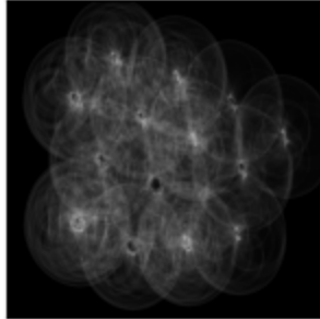
Radius 45
