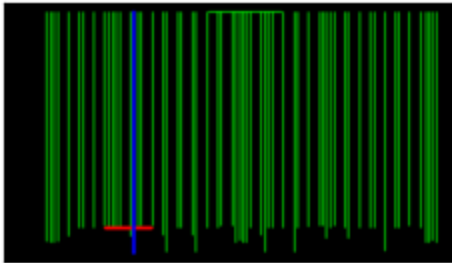
Segments
