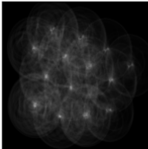
Radius 55
