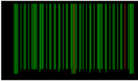
OpenCV lines
