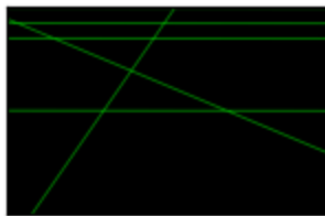
Lines
