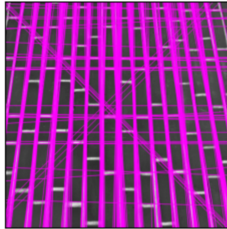
brick overlay
