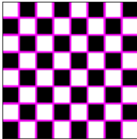
checkerboard overlay
