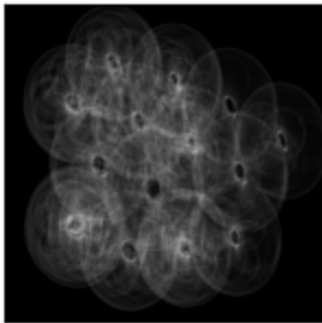
Radius 40
