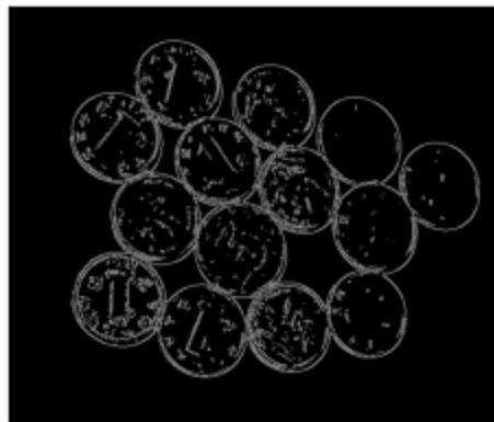
Edges
