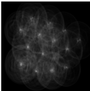
Radius 55
