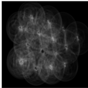
Radius 45
