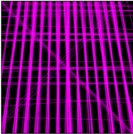
brick lines
