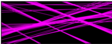
text lines
