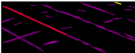
text segments
