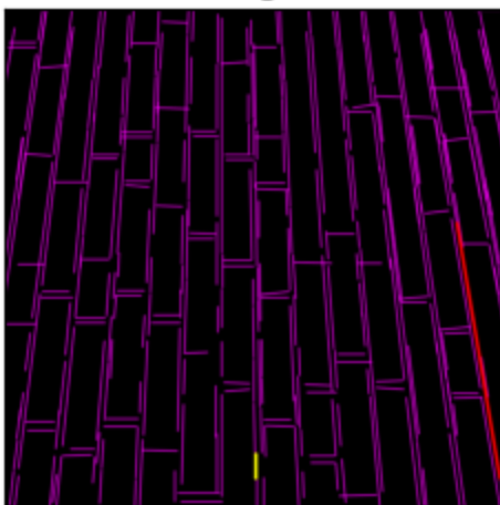
brick segments
