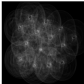
Radius 60
