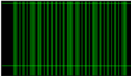
OpenCV lines
