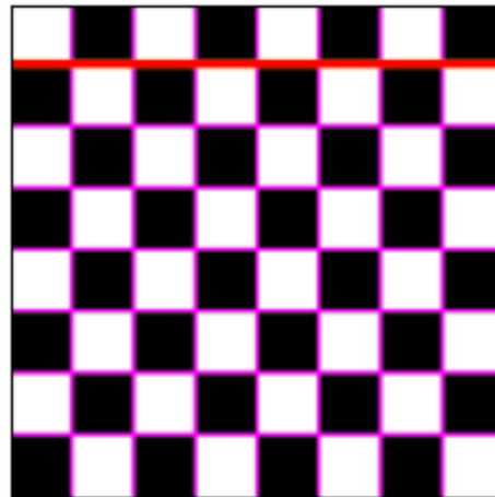
checkerboard overlay
