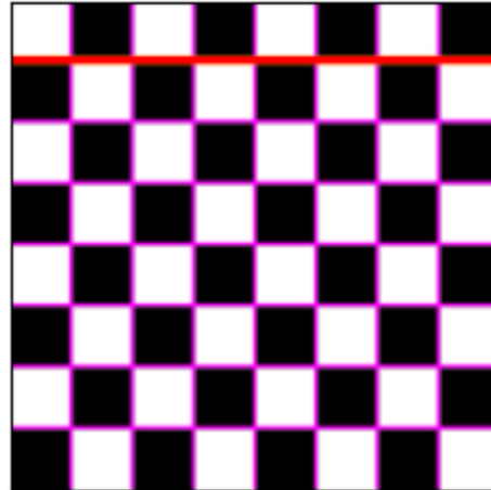
checkerboard overlay
