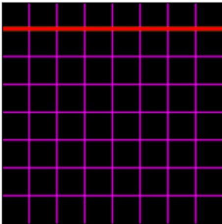
checkerboard segments
