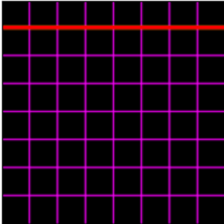
checkerboard segments
