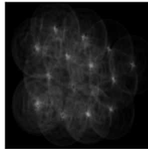
Radius 50
