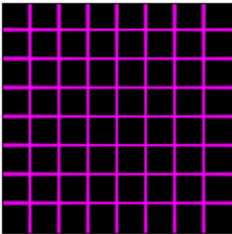
checkerboard lines
