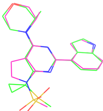
Figure: one bioisostere possess a pyrrolo pyrimidine scaffold (in magenta). It is aligned on the input structure 7jjg_B_VCD.sdf (in green). The fitness score gfit+hfit = 1.54 . It has the same molecular structure as AD1058.sdf.
