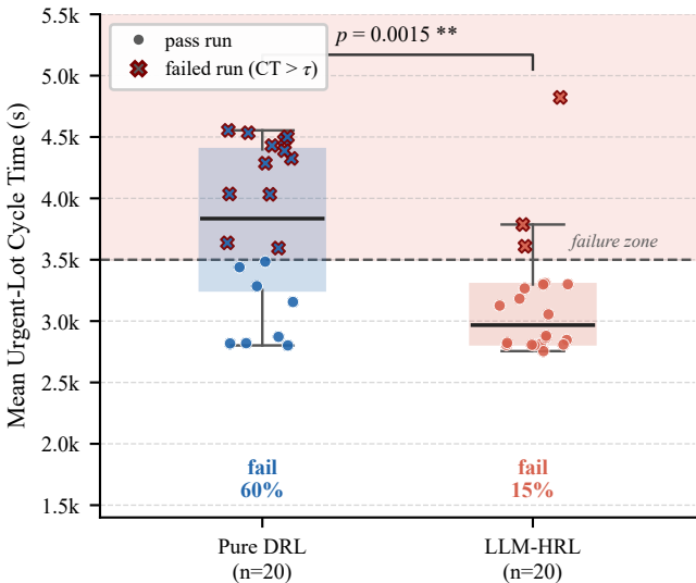
Reliability across 20 independent seeds
