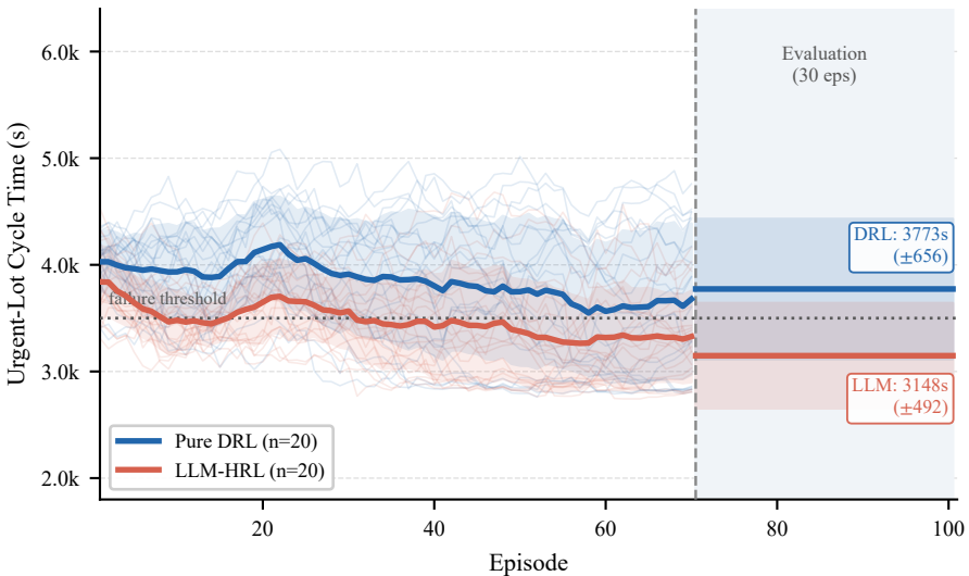
Training convergence and evaluation (shaded band = \pm 1 SD)
