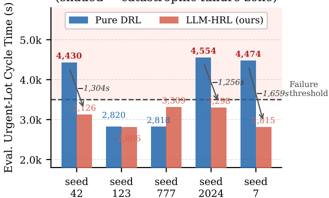
Per-Seed Results at 20 Urgent Lots (shaded = catastrophic failure zone)
