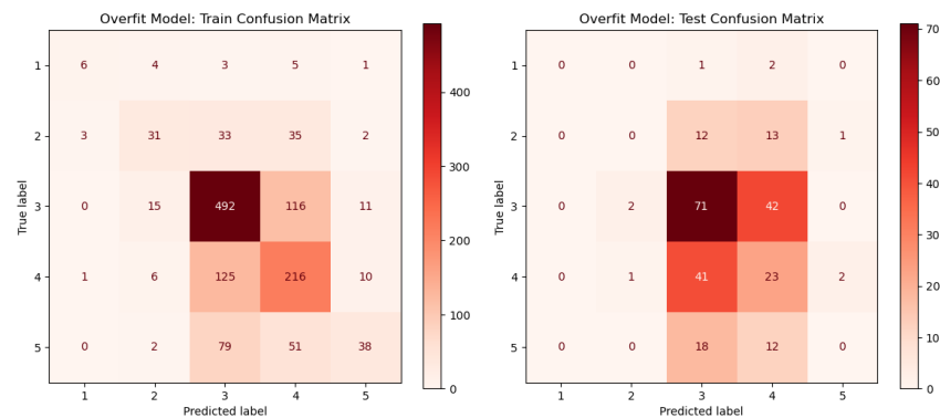
Figure 24: Multi-Layer Perceptron: overfit model confusion matrix (train vs test).
