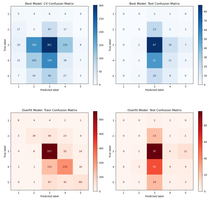
Figure 23: Gradient Boosting Classifier: overfit model confusion matrix (train vs test).
