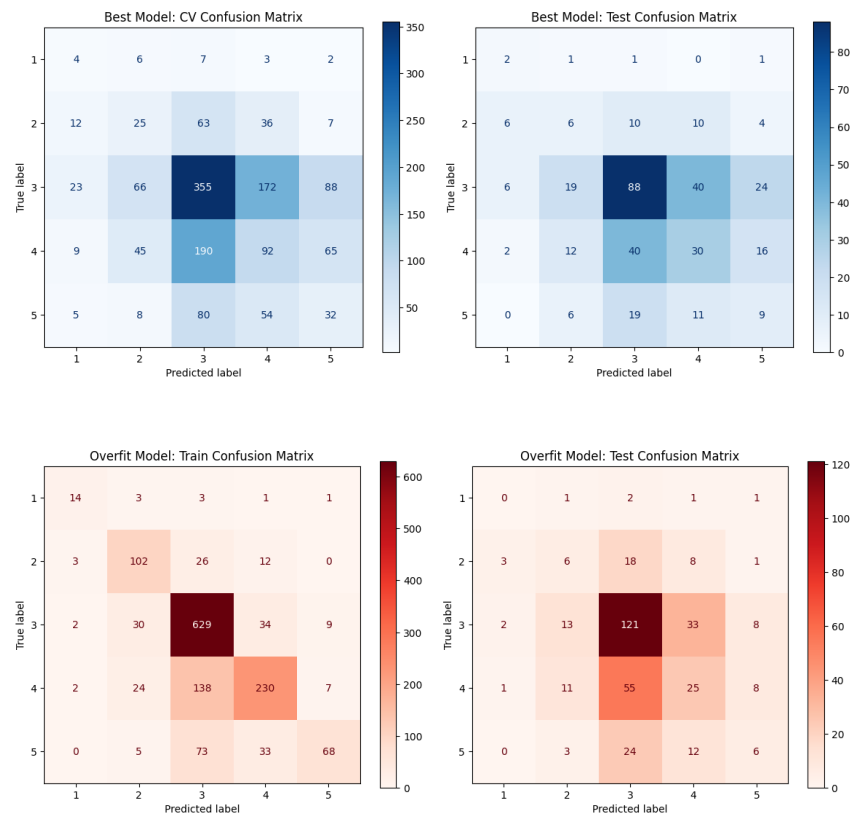
Figure 22: Random Forest Classifier: overfit model confusion matrix (train vs test).
