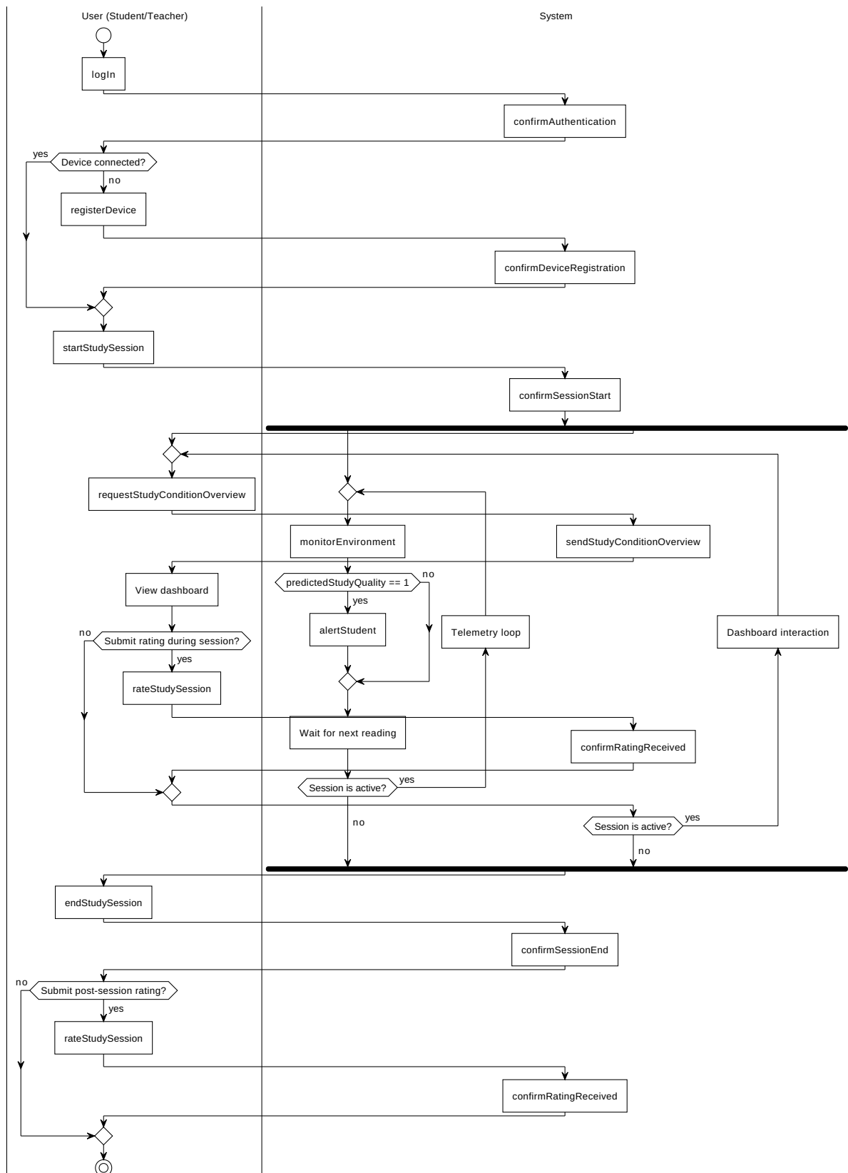
Activity Diagram: StudyHelper Global Workflow
