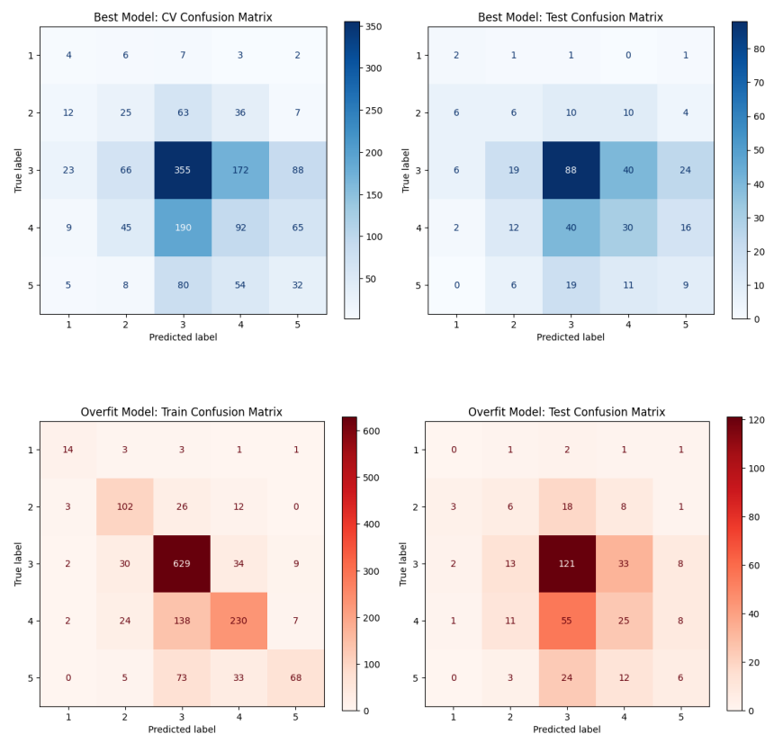
Figure 17: Random Forest Classifier: overfit model confusion matrix (train vs test).
