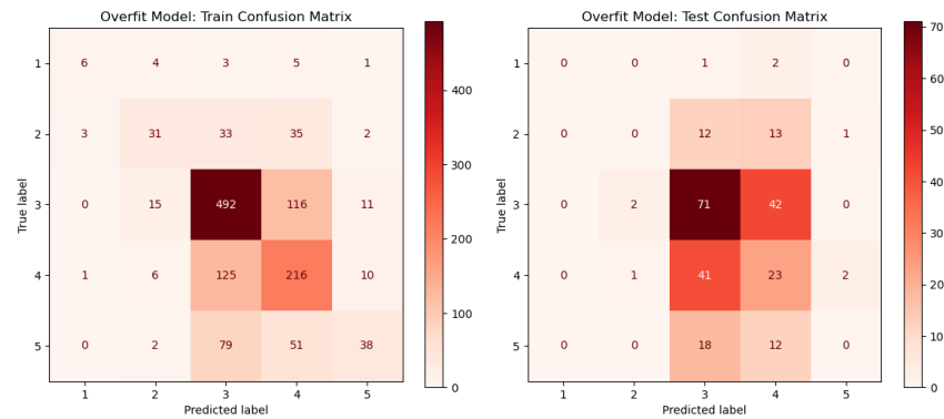
Figure 19: Multi-Layer Perceptron: overfit model confusion matrix (train vs test).
