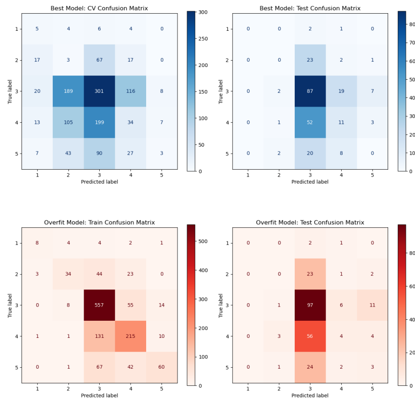
Figure 18: Gradient Boosting Classifier: overfit model confusion matrix (train vs test).
