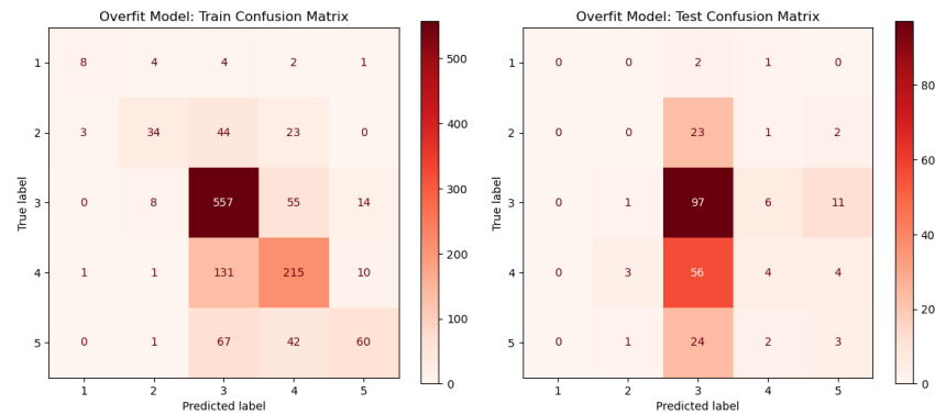
Figure 18: Gradient Boosting Classifier: overfit model confusion matrix (train vs test).
