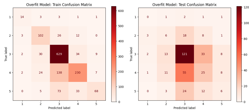
Figure 17: Random Forest Classifier: overfit model confusion matrix (train vs test).
