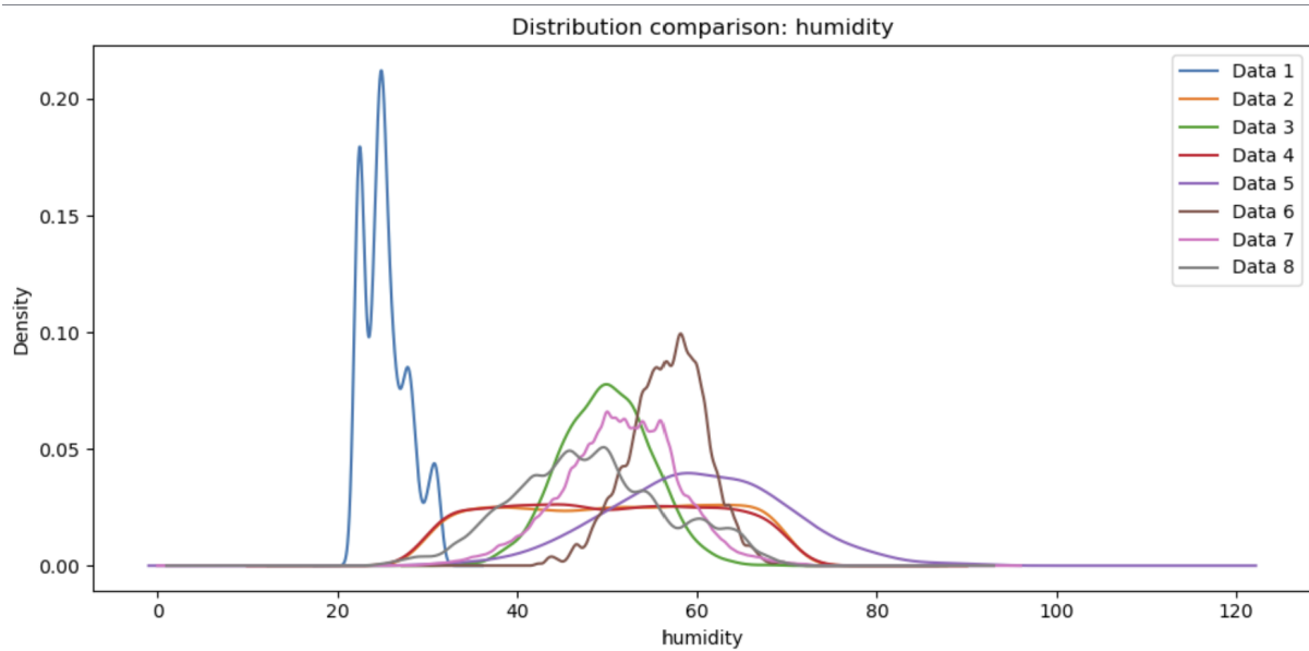
Figure 11: Suspiciously perfect feature distributions in candidate datasets.
