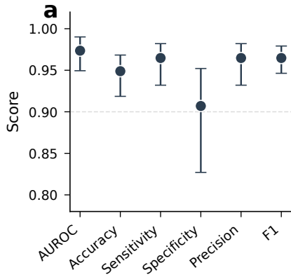
Cancer Detection Metrics
