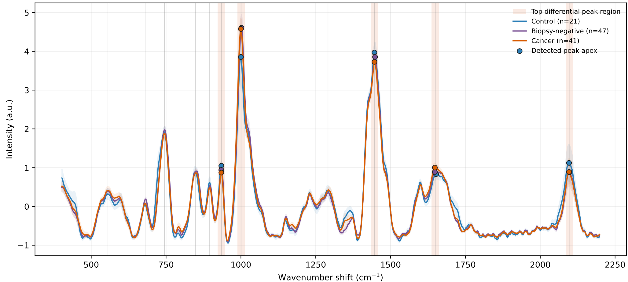
Fig04b. 3-group peak sets: Control / Biopsy-negative / Cancer
