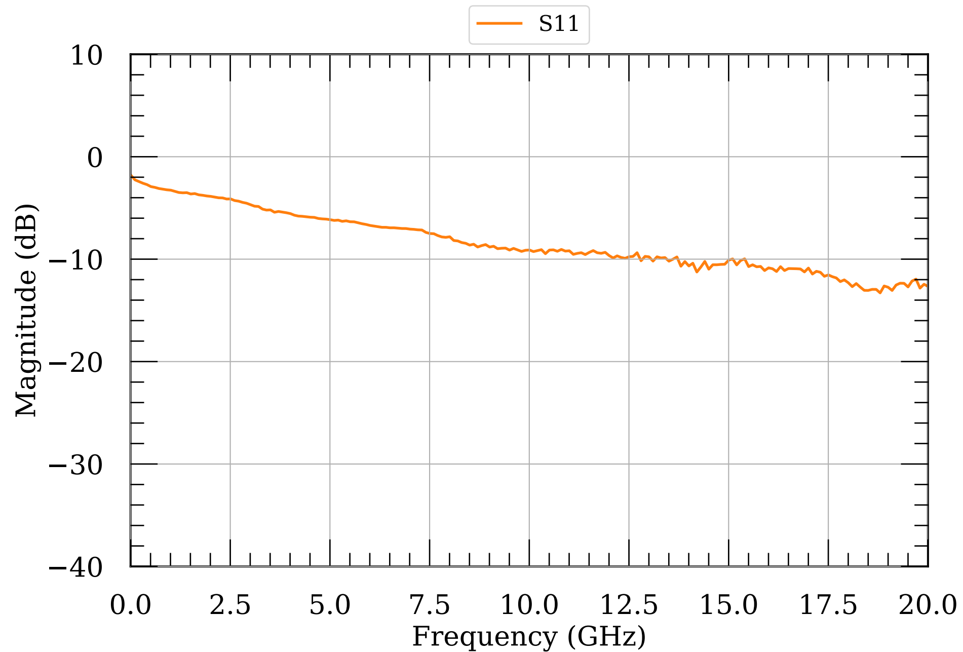
LNA S-params 0.0
