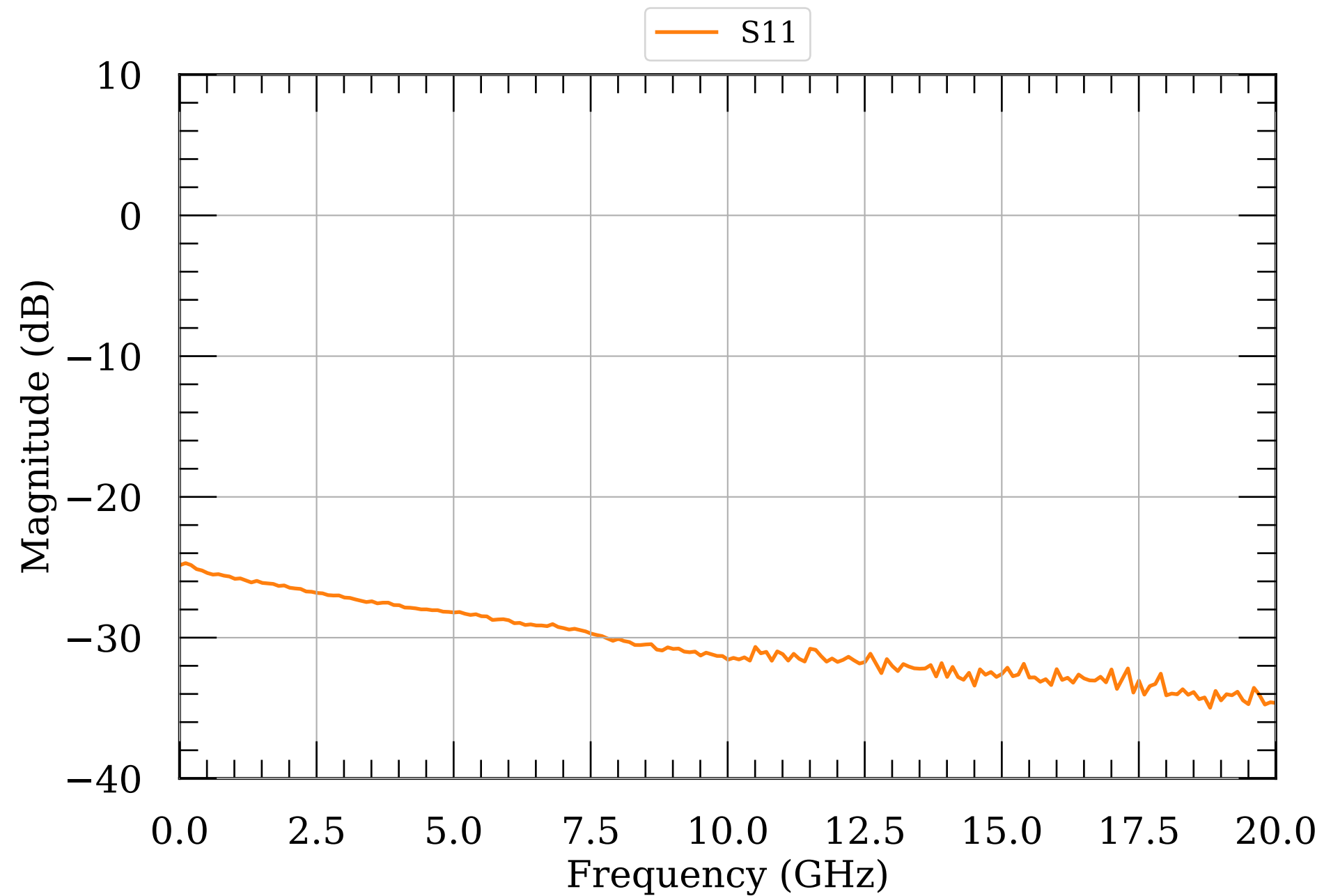
LNA S-params 13.0
