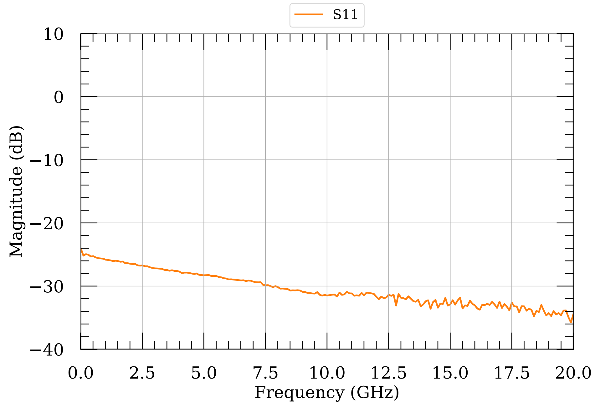
LNA S-params 13.5
