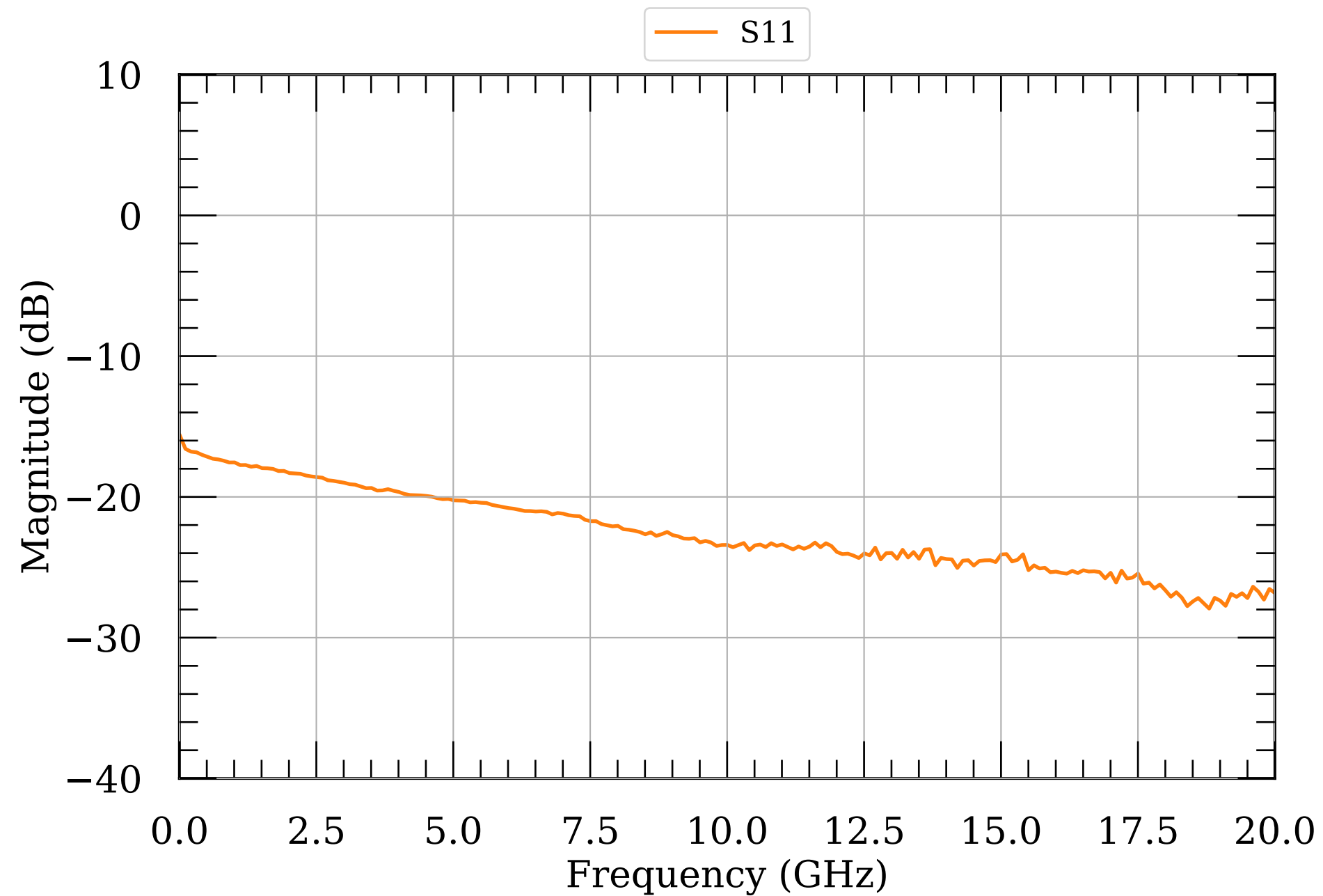
LNA S-params 14.5
