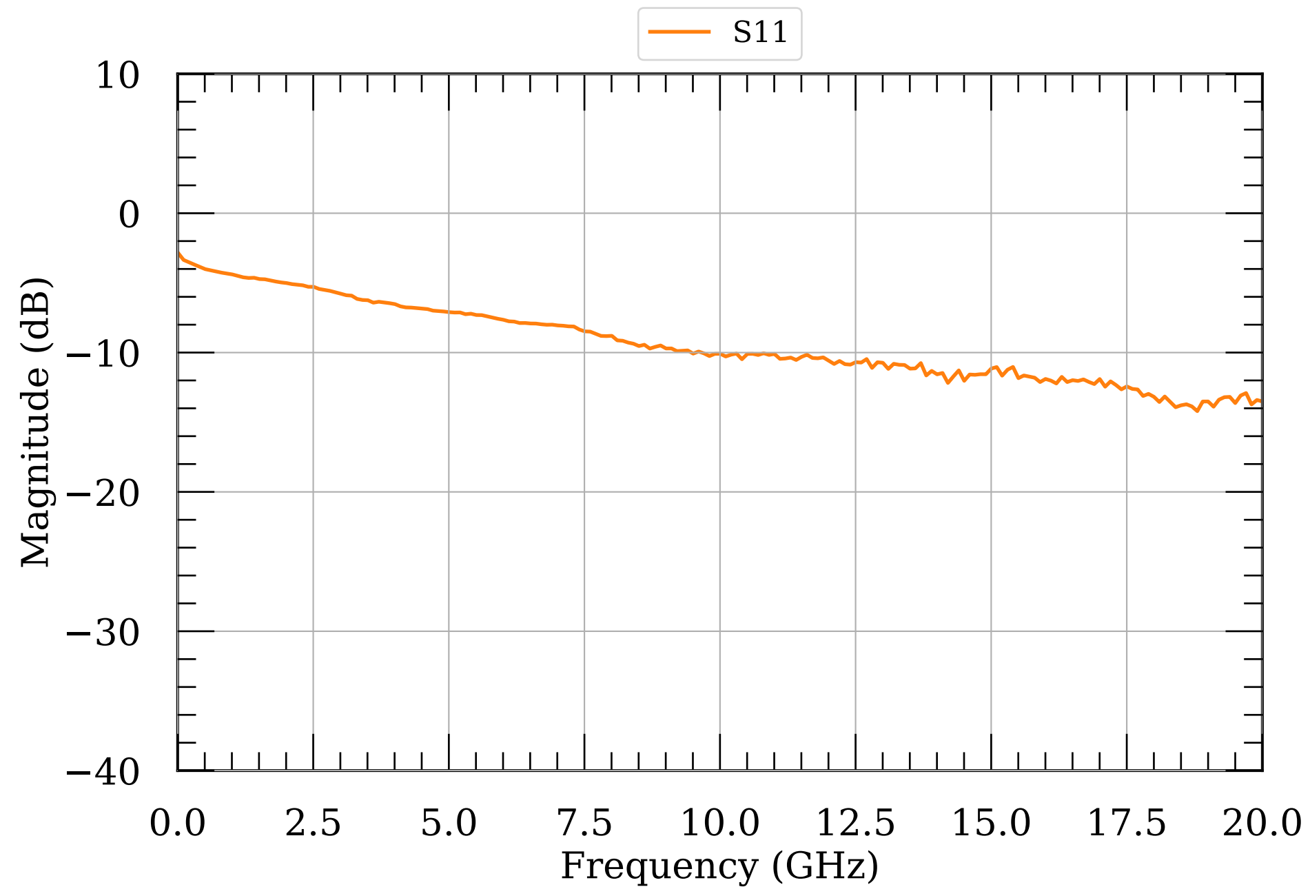
LNA S-params 16.5
