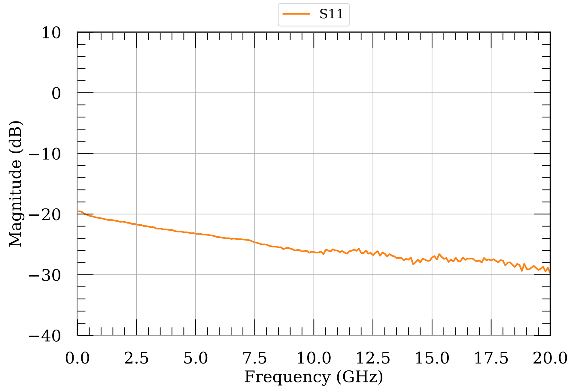
LNA S-params 17.0
