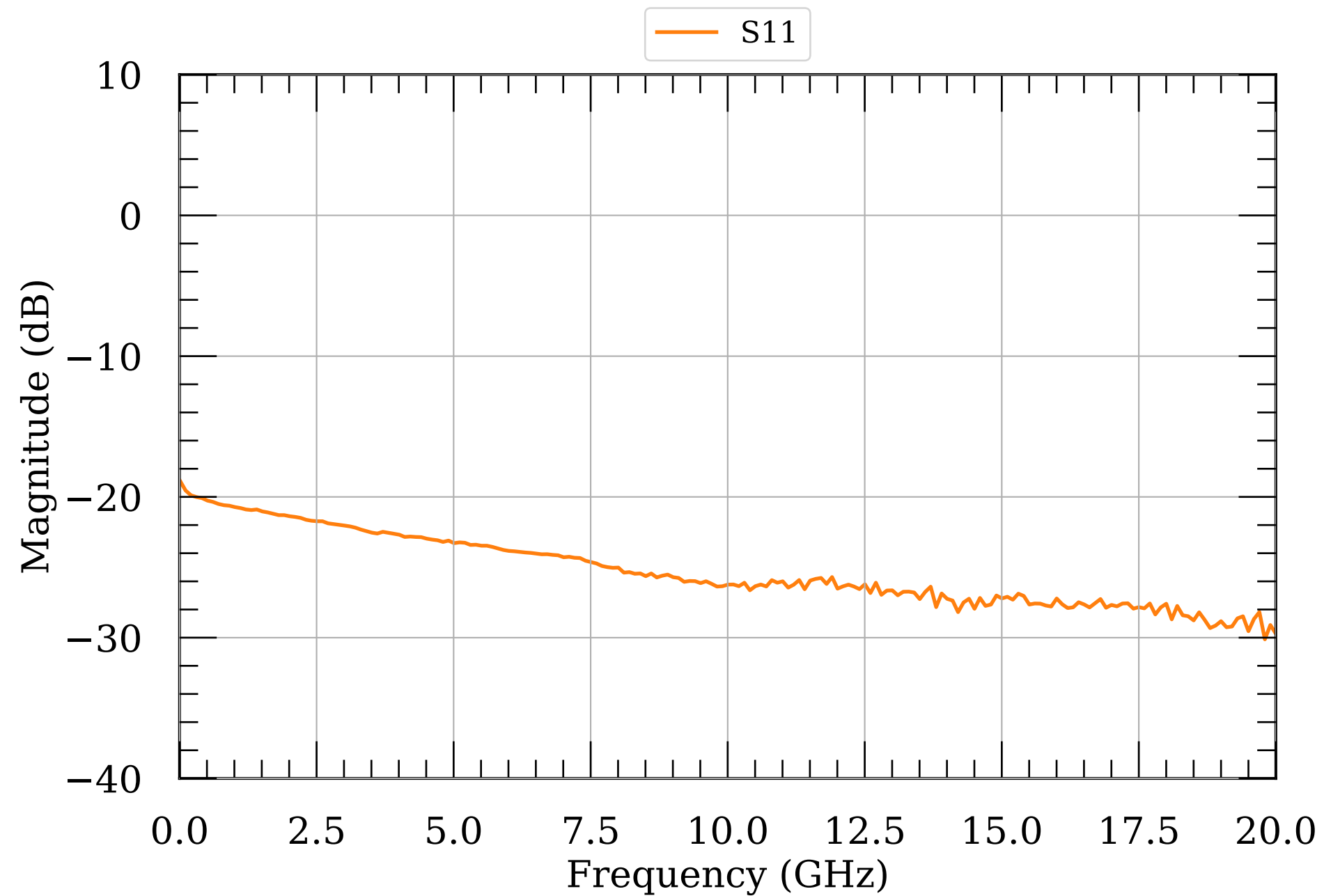
LNA S-params 17.5
