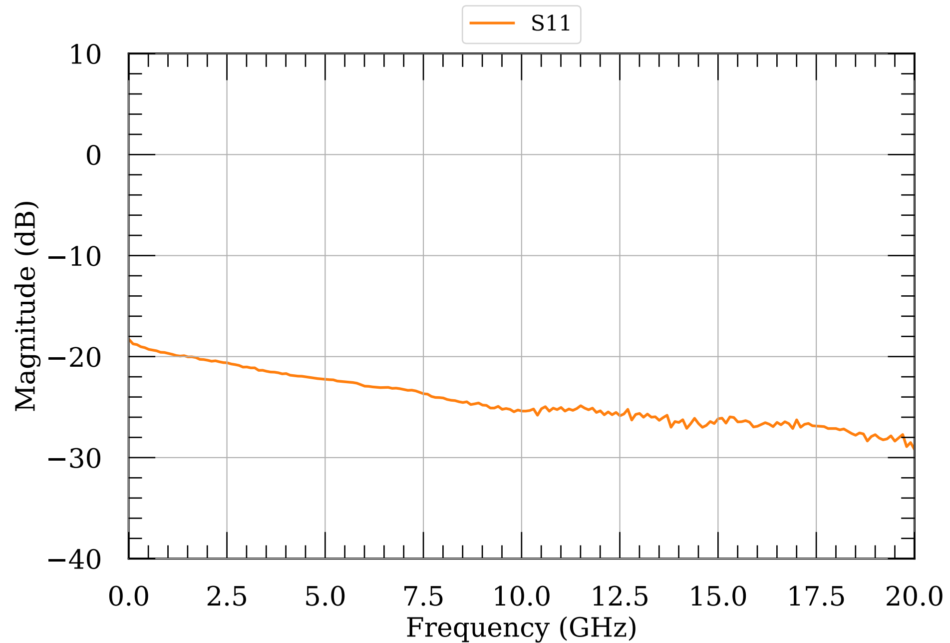
LNA S-params 1.0
