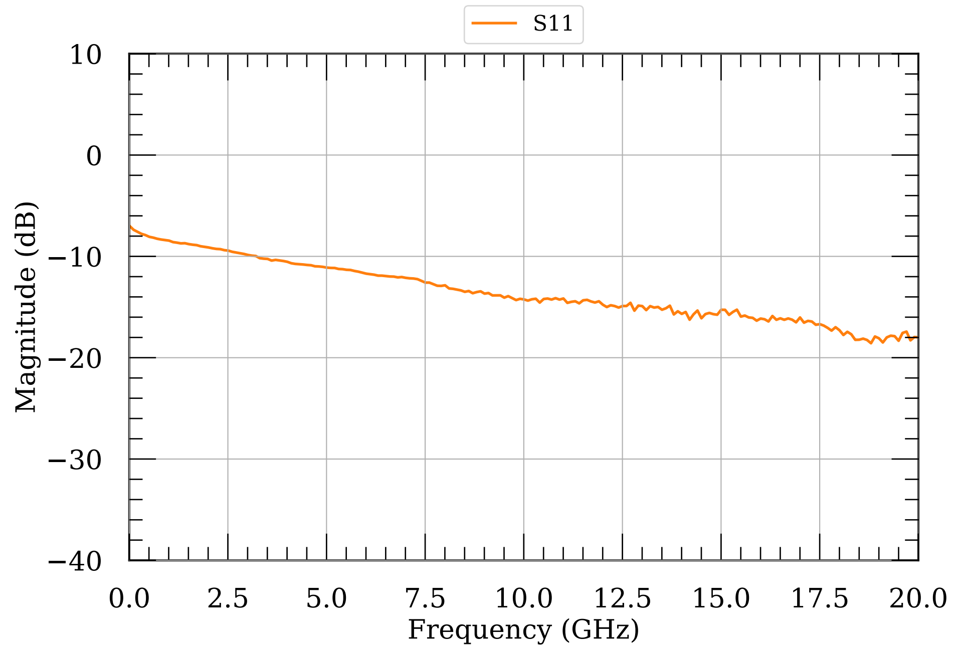
LNA S-params 20.0
