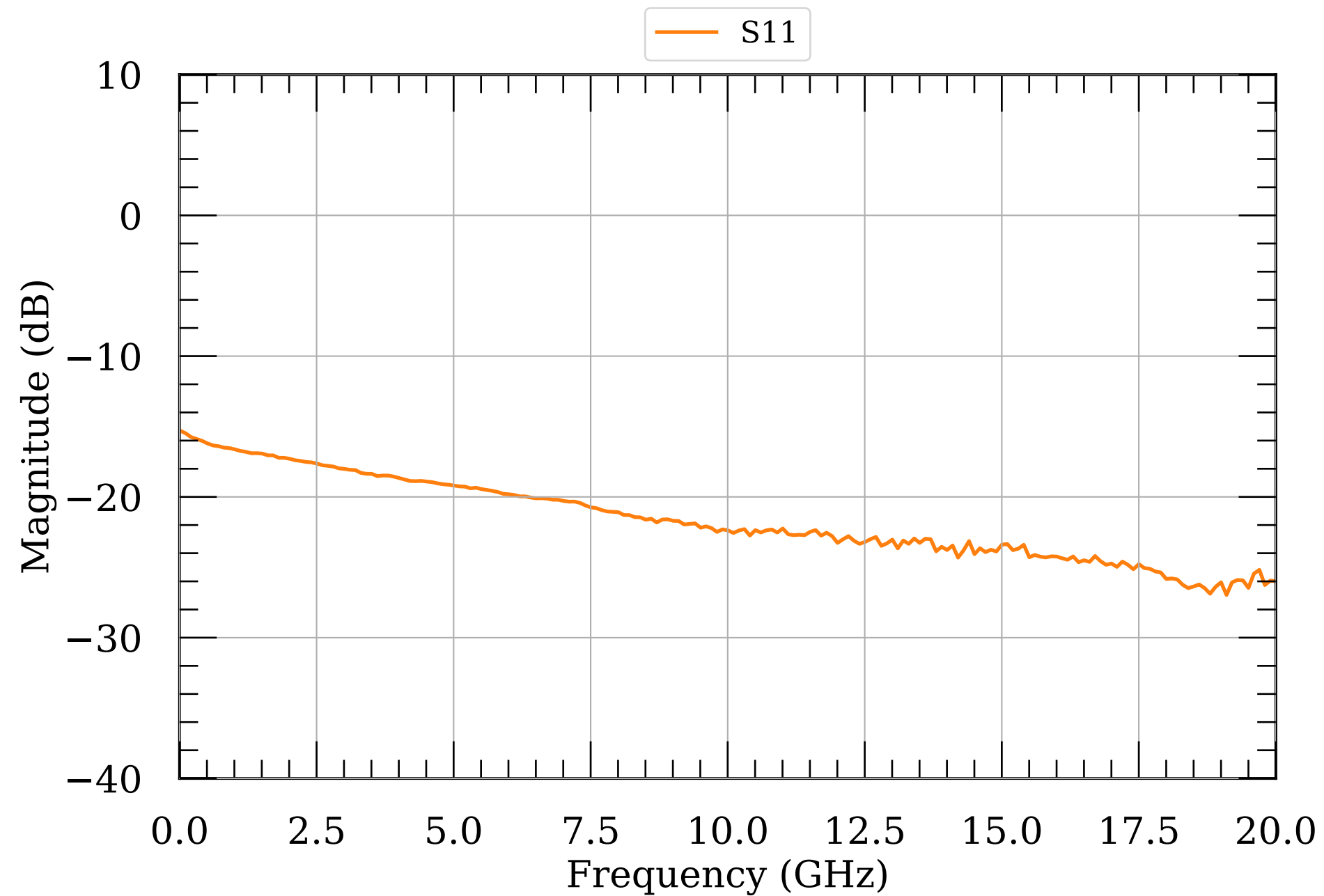
LNA S-params 22.5
