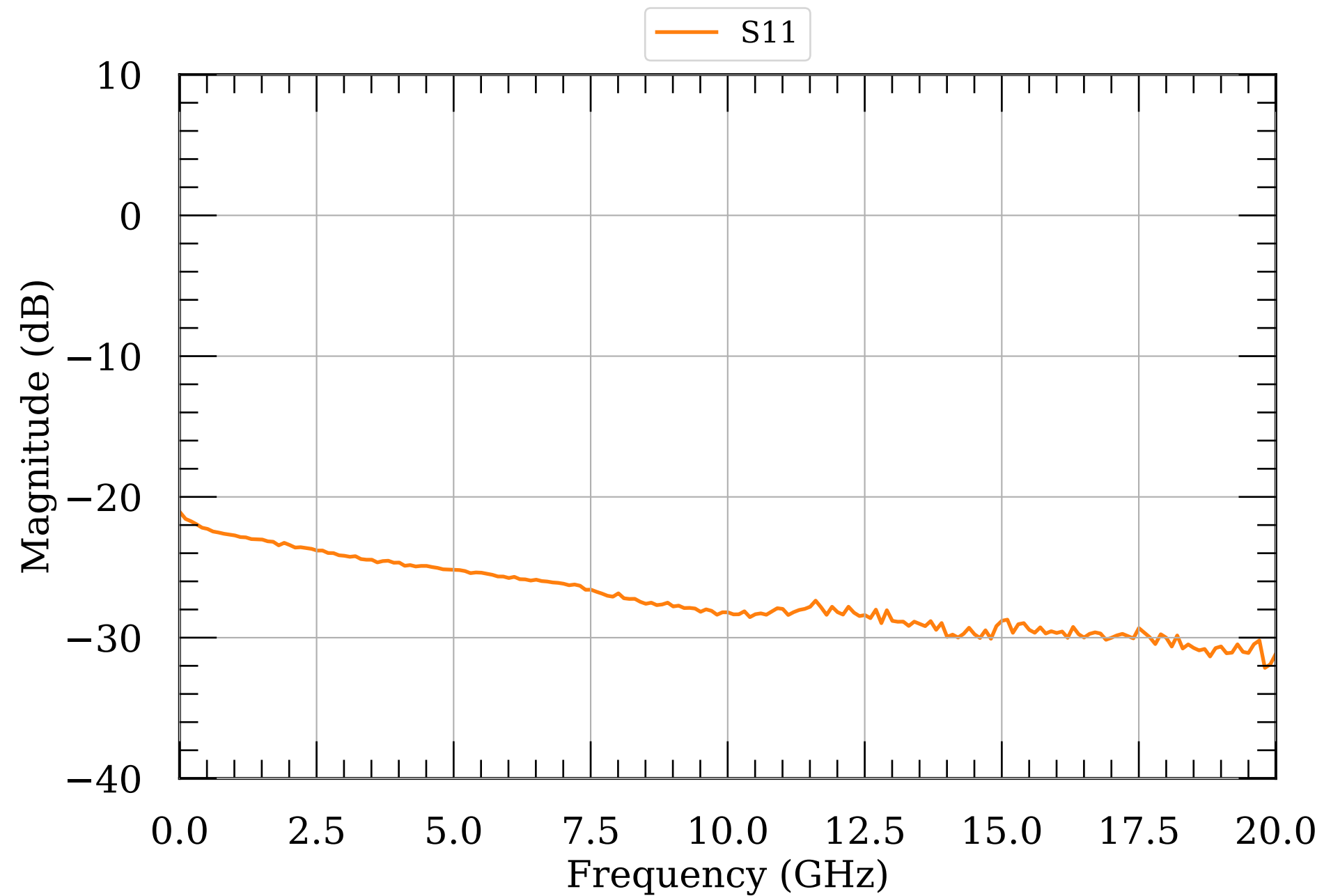
LNA S-params 25.5
