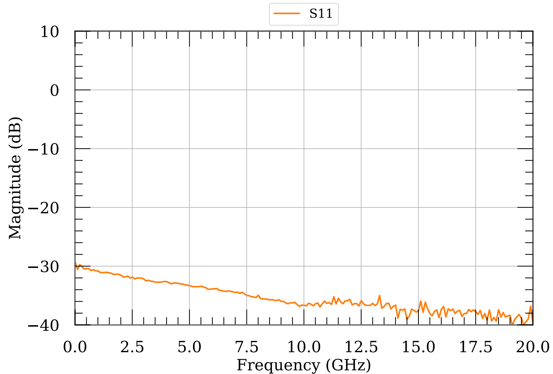
LNA S-params 27.5
