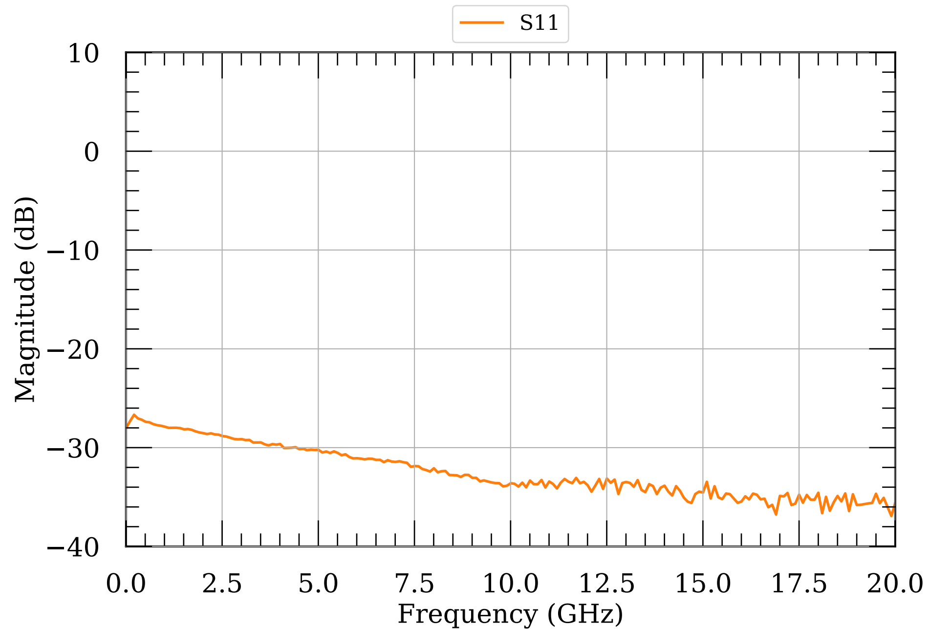
LNA S-params 3.5
