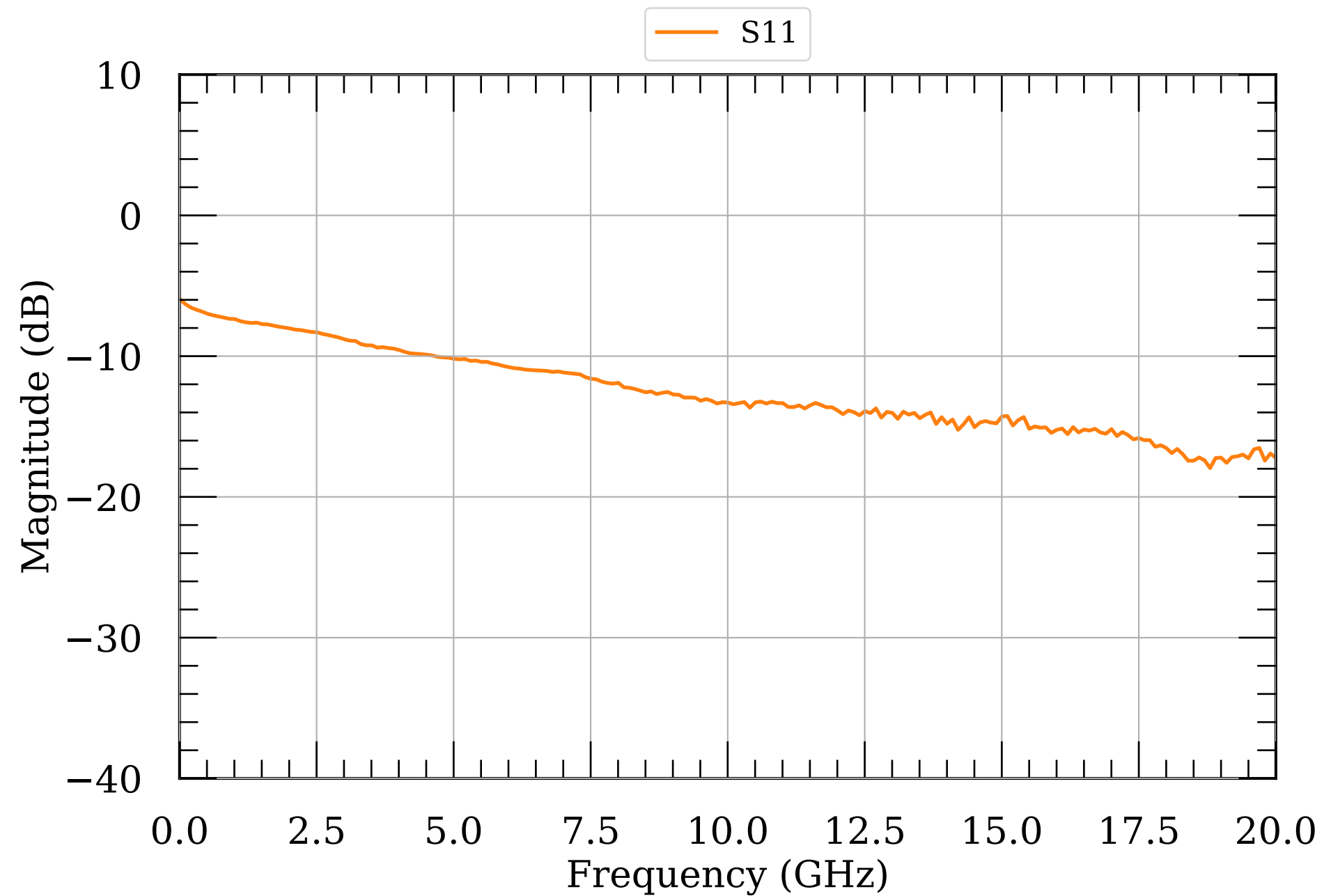
LNA S-params 4.0
