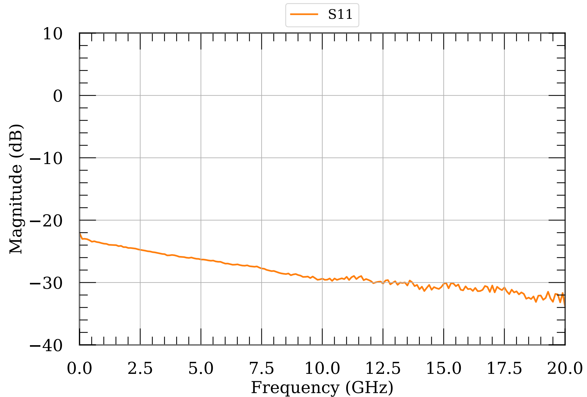
LNA S-params 5.0
