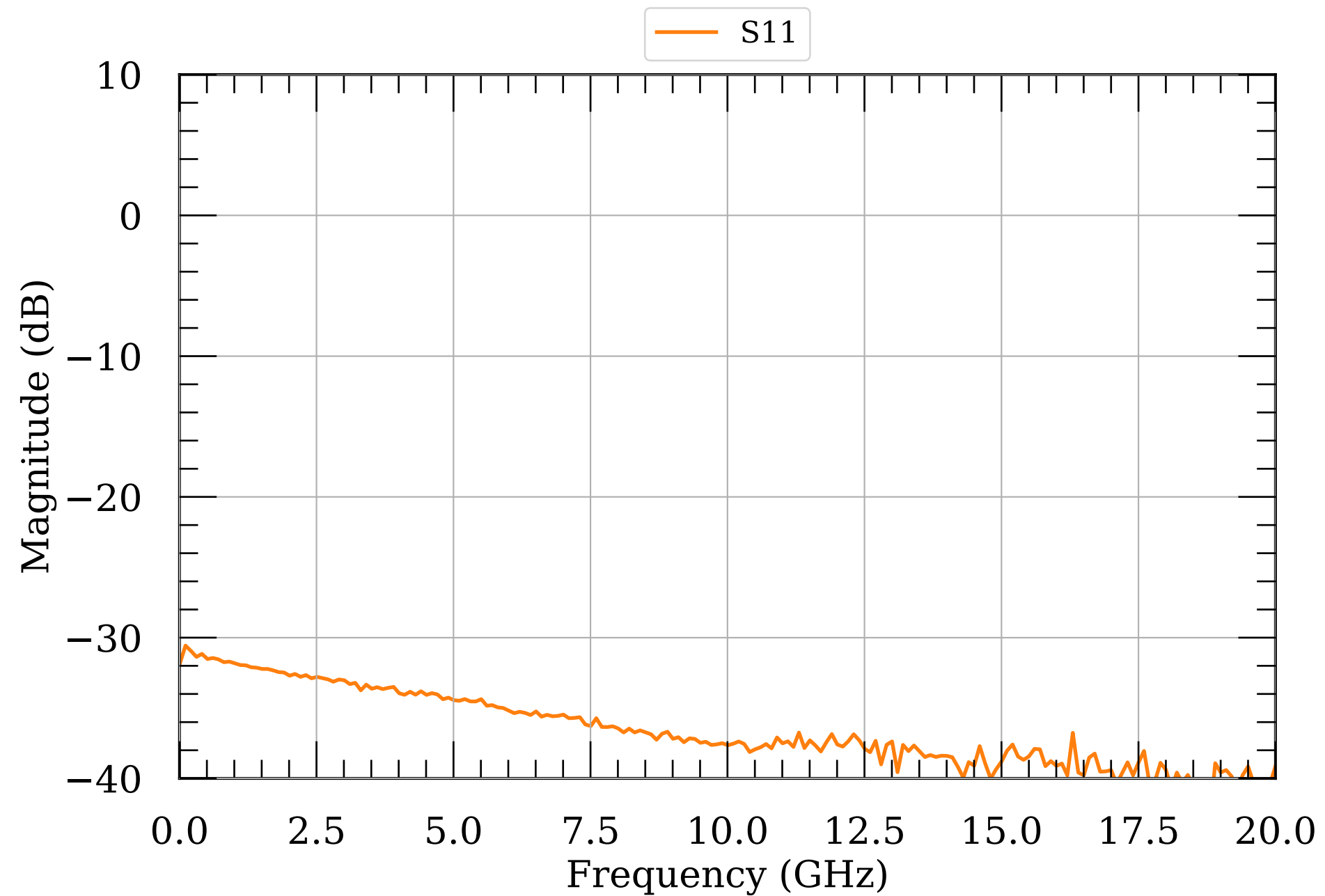
LNA S-params 7.5
