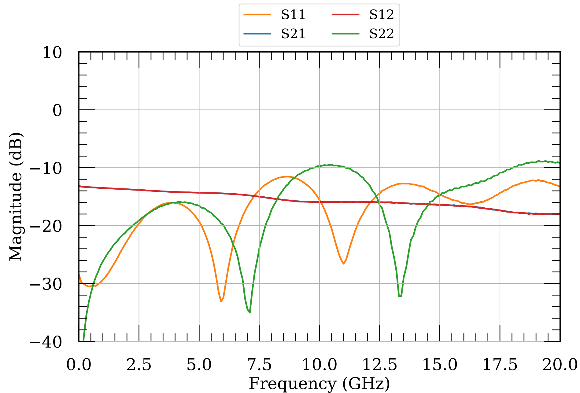
LNA S-params, 11 dBm
